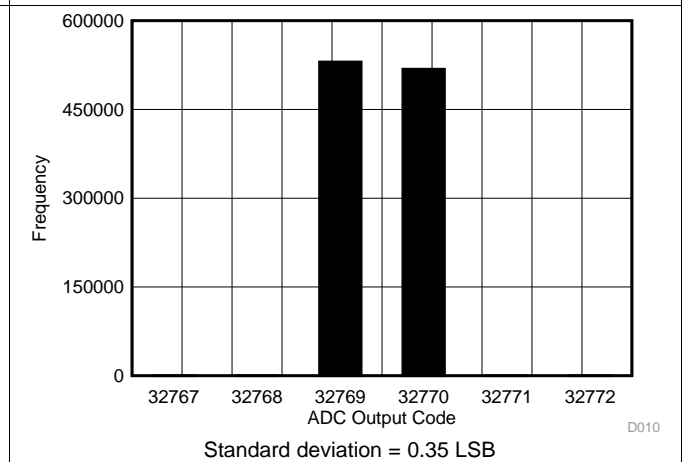
Figure 16. DC Input Histogram, Code Transition
