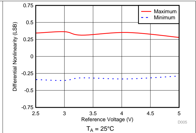
Figure 14. DNL vs Reference Voltage
