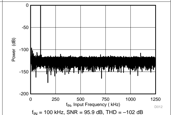
Figure 18. Typical FFT
