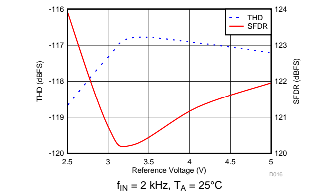
Figure 22. Distortion Performance vs Reference Voltage
