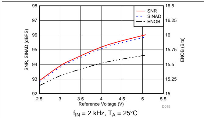
Figure 21. Noise Performance vs Reference Voltage
